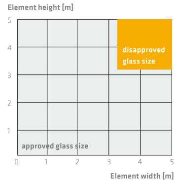
Fig. 11: Under the same conditions as in Fig. 10 the facade elements can be much bigger with Sikasil SG-550. Vice versa the joint bite for the same element sizes can be 30 % smaller and the total joint volume even 60 % lower
