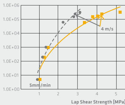
Fig. 31: The higher the impact speed, the higher the adhesives' shear strength, the higher the design stress.
