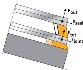
Fig. 13: Deflection of SG and IG joints under permanent tension and shear due to displacement and rotation after installation.
