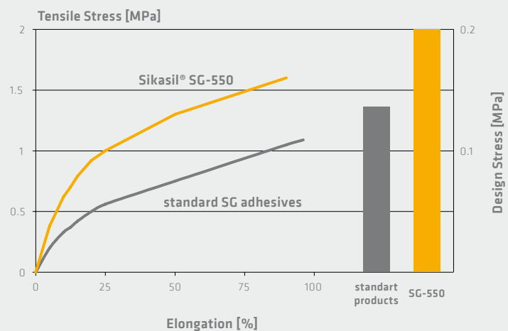
Fig. 8: Comparison of tensile stress and design strength of Sikasil® SG-550 with standard SG adhesives
