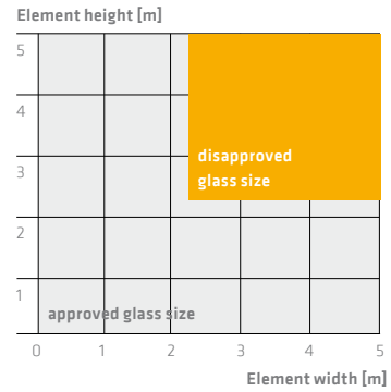
Fig.10: Feasible SG element size with Sikasil SG-500 SG Joint Dimension: 12 mm x 6mm; wind load: 1.50 kPa; dead load supported
