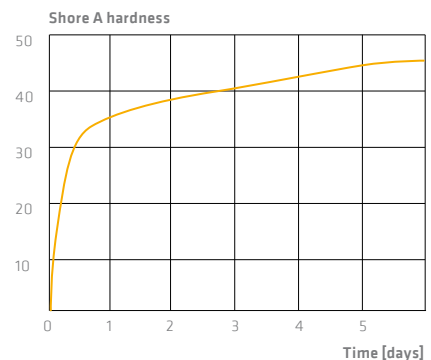
Fig. 6: Shore A hardness in the curing of two-component silicones, such as Sikasil® SG-500 or Sikasil® IG-25, as a function of time
