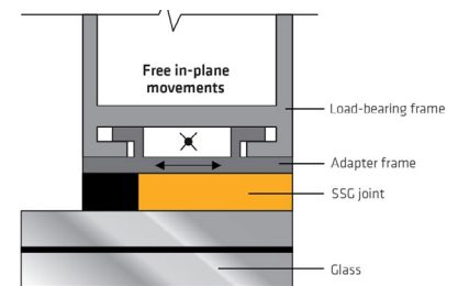
Fig. 14: Slim adapter frame, free to rotate and slid
