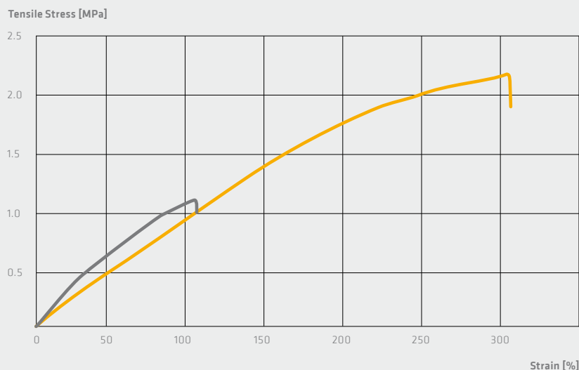
Fig. 7: Stress-strain curve, comparison of H-specimens and dumbbell
