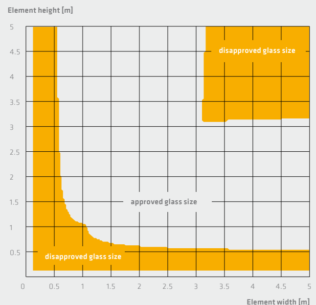
Fig. 18: Under the same conditions as in Fig. 17, the IG units can be much bigger with Sikasil® IG-25 HM Plus. Vice versa the seal height for the same unit sizes can be 25 % smaller.
