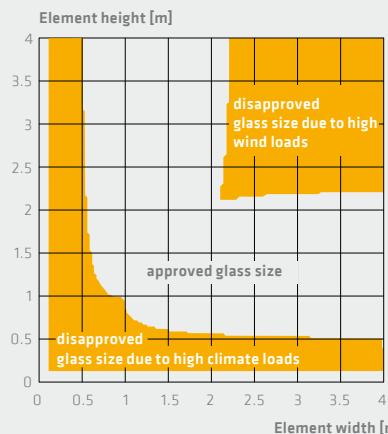
Fig. 20 Climatic and wind loads are relevant for sealant height calculation
