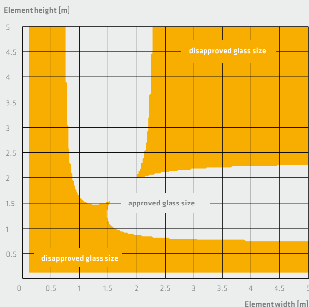
Fig. 17: Feasible triple glazed IG unit with Sikasil® IG-25, IG configuration 8/10/4/10/8 IG Joint dimensions 10 mm x 6 mm
