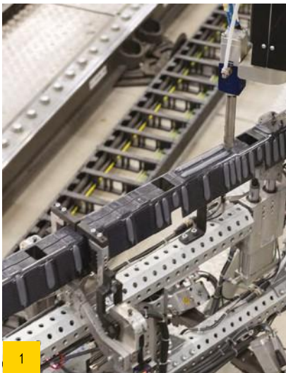
1 Central tunnel bonding (CFRP - steel) 2 Rocker bonding (CFRP - steel)
